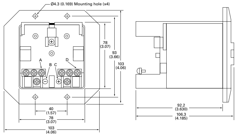
IC800ABK001 Absolute encoder battery pack
