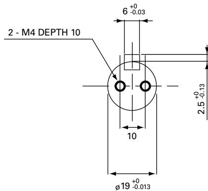
Shaft detail
